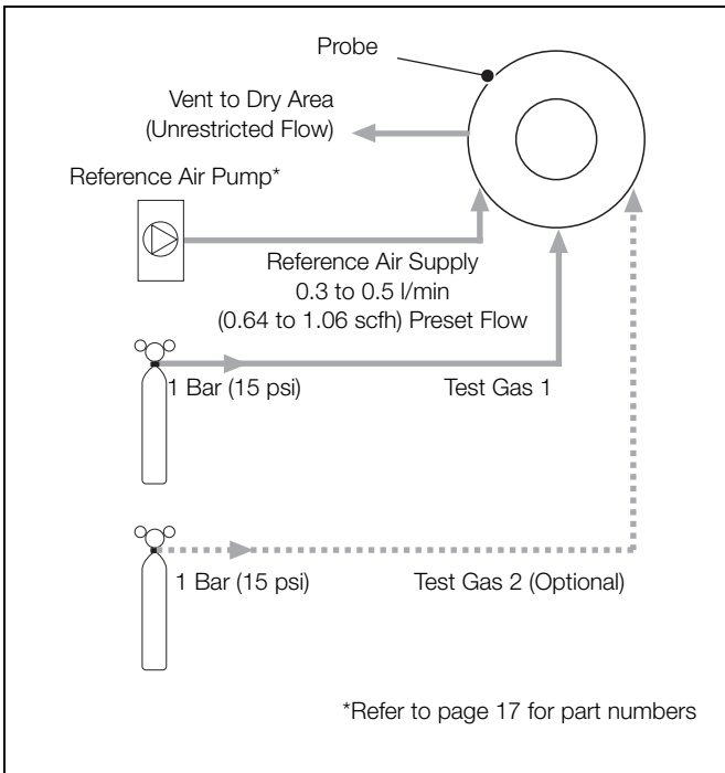
AutoCal with Test Gas(es) and Restrictors
